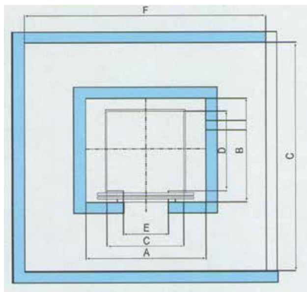
Hoist Machine Room Plan For Auto Door
